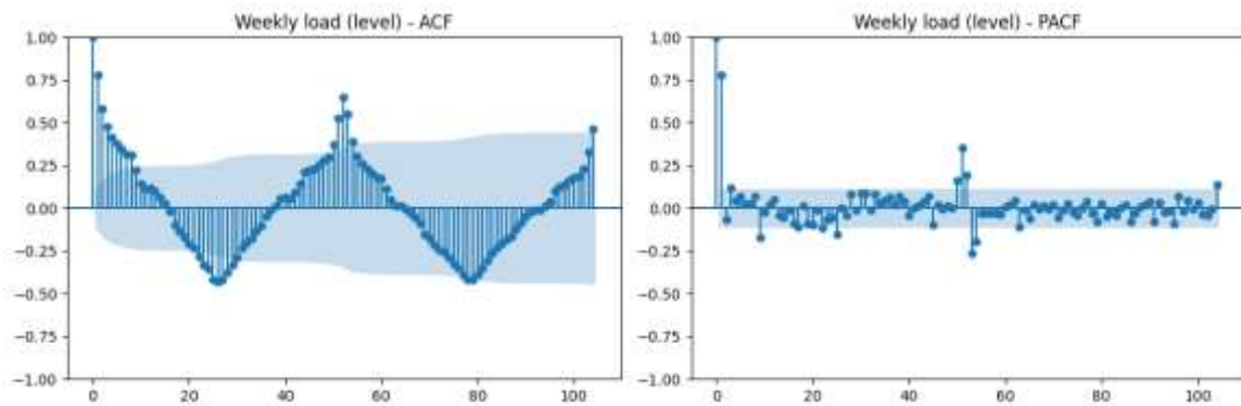
Figure 3. Weekly load ACF/PACF in levels, showing strong annual dependence.
